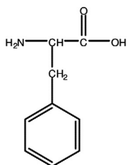
L-phenylalanine
